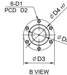
B VIEW
